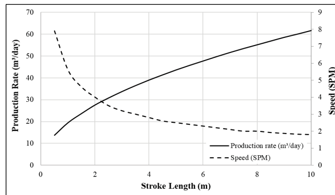
Figure 11: Effect of the stroke length.
