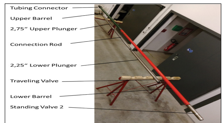
Figure 15: 2.75/2.25 inches x 1.5 m hydraulic pump prototype.
