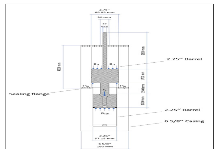
Figure 16: Pump setup for testing.
