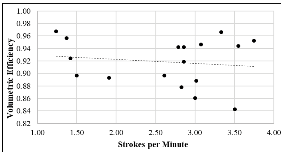
Figure 19: Volumetric pump efficiencies test case 1 to 3.
