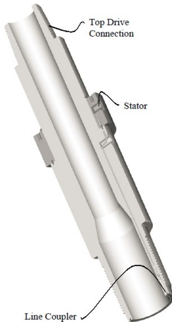
Figure 6: A top drive sub provides a communication link between the rotating drill string and a data acquisition system (Jellison et al., 2003).
