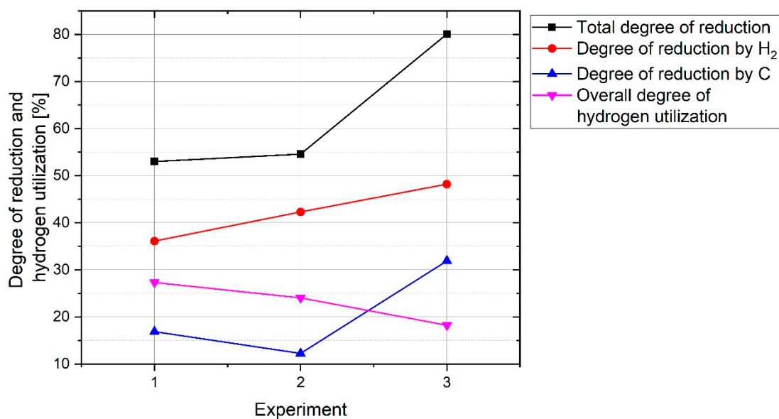
Figure 17. Degree of reduction and hydrogen utilization of Experiments 1, 2 and 3.
