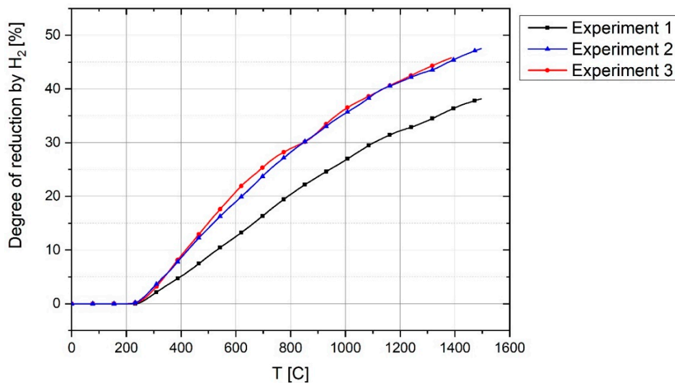
Figure 16. The degree of reduction of iron oxide in Experiments 1, 2 and 3.
