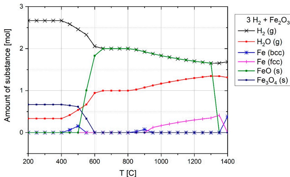
Figure 13. Chemical composition of 3 mol H 2 and 1 mol Fe 2 O 3 at equilibrium and 1 atm pressure.
