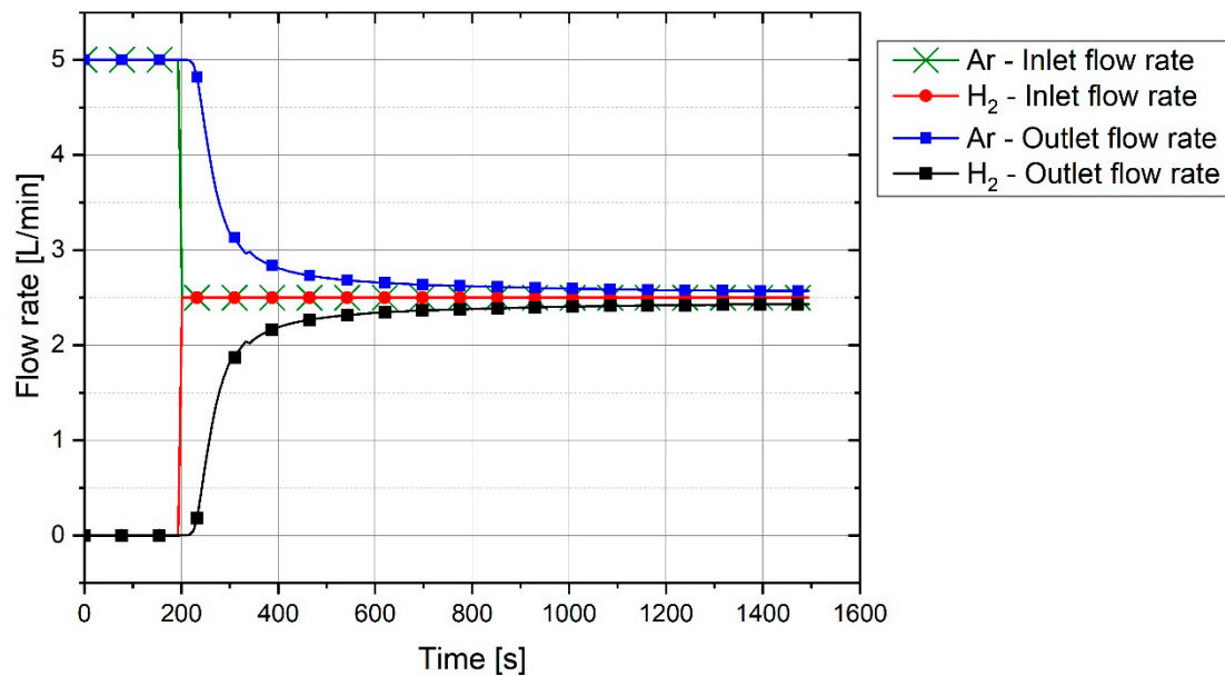
Figure 4. Reference flow rate of a premixed 50% Ar/50% H 2 gas with a total flow rate of 5 L/min.
