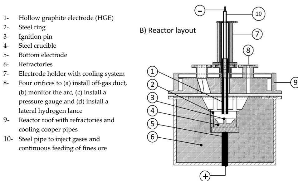
Figure 1. Schematic of laboratory-scale plasma facility at Montanuniversitaet Leoben: (A) process flow diagram and (B) reactor layout [10].
