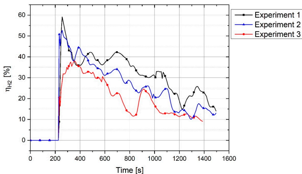
Figure 14. \eta_{H_2} of Experiments 1, 2 and 3.
