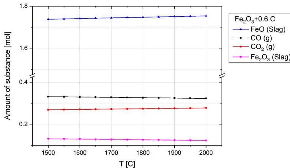
Figure 11. The composition of 0.6 mol of carbon and one mol of haematite at equilibrium over temperature.
