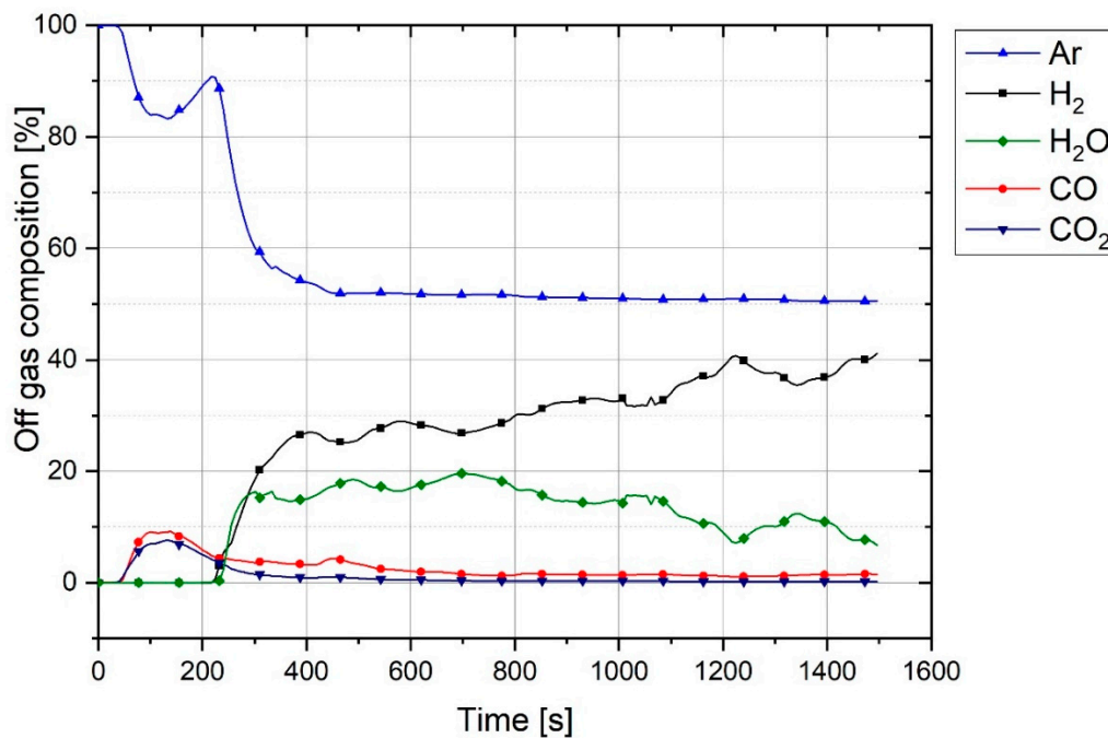
Figure 6. Chemical composition of off-gas from Experiment 1.
