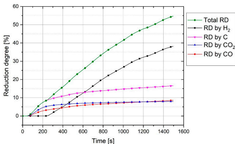
Figure 10. Degree of reduction by the production of CO, CO 2 and H 2 O and total degree of reduction of Experiment 1.
