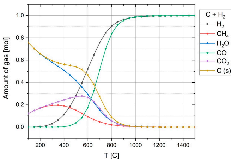
Figure 7. Composition of 1 mol C and 1 mol H 2 O at equilibrium at 1 atm pressure over temperature.
