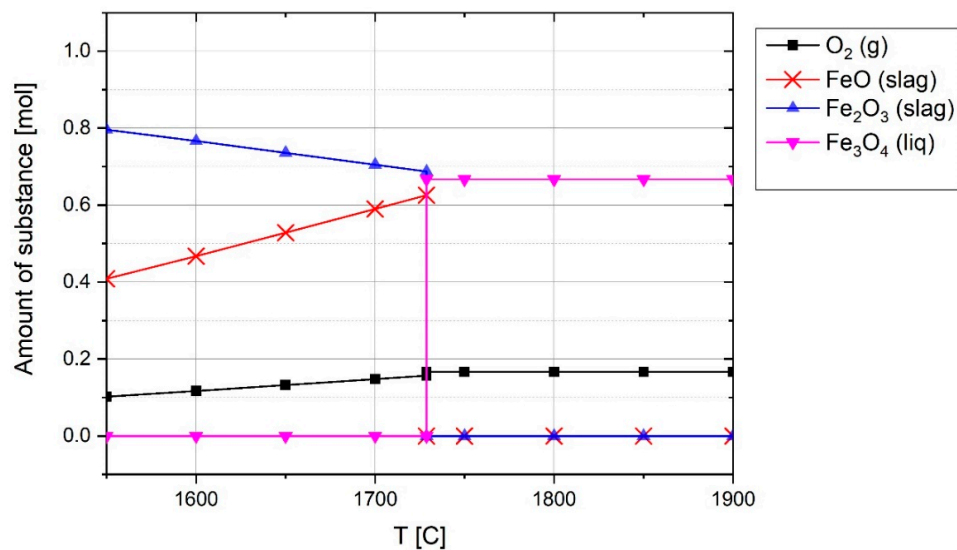
Figure 9. Chemical composition of 1 mol haematite over temperature at equilibrium at 1 atm pressure.
