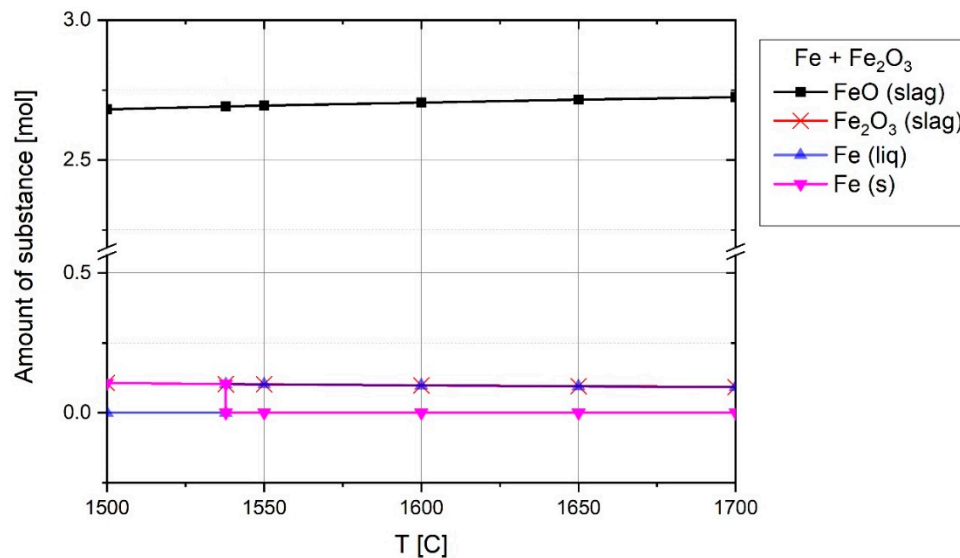
Figure 8. Chemical composition of 1 mol Fe and 1 mol of Fe 2 O 3 at equilibrium at 1 atm pressure above melting temperature, FactSage TM 7.2 (Database: FactPS and FToxide (2018)).
