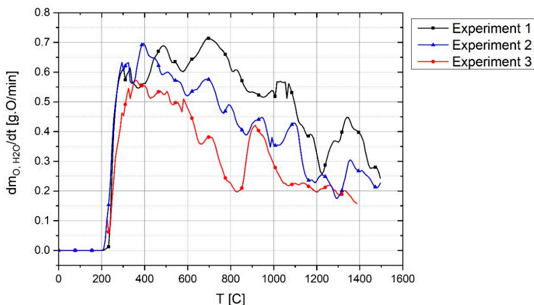
Figure 15. Reduction rate by hydrogen in Experiments 1, 2 and 3.
