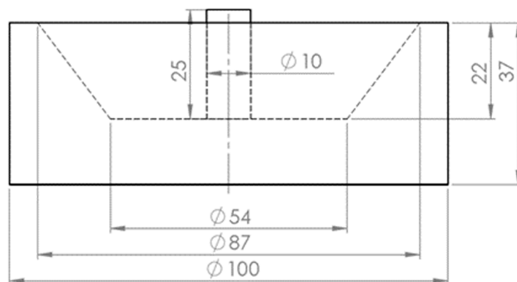
Figure 2. Drawing of the steel crucible, dimensions are in mm.
