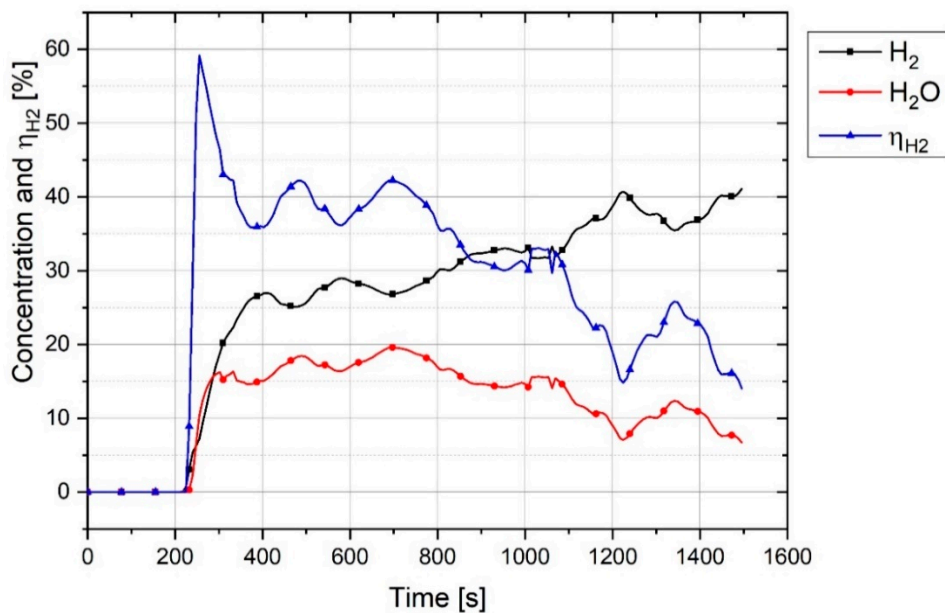
Figure 12. H 2 and H 2 O concentration in off-gas and \eta_{H_2} of the Experiment 1.
