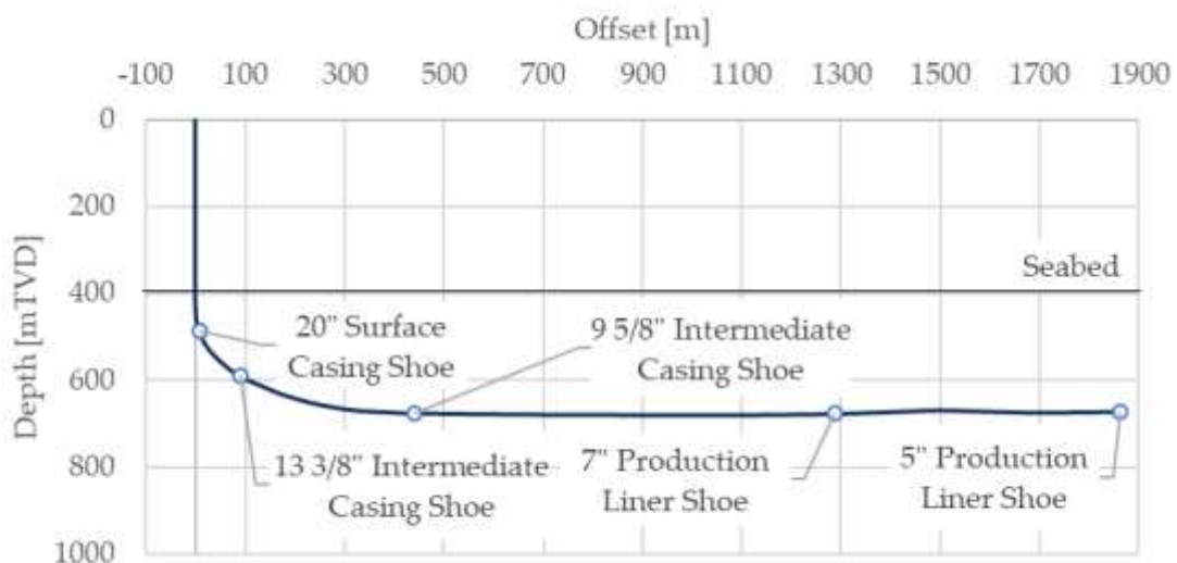
Figure 4: Wisting Central II trajectory profile
