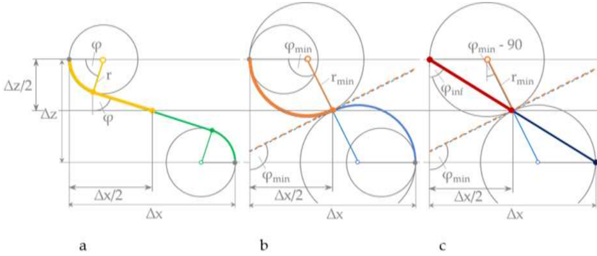
Figure 18: Sheave model for J-shaped trajectory
