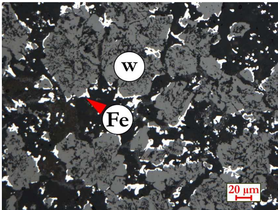
Figure 53: Iron sparks (whisker) grown at the edges of wuestite (dark grey).
