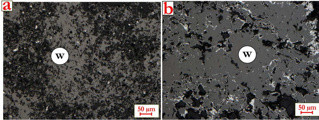
Figure 52: a) Wuestite (w) with metallic iron specks (white); b) Wuestite (w) with metallic iron shell (white).
