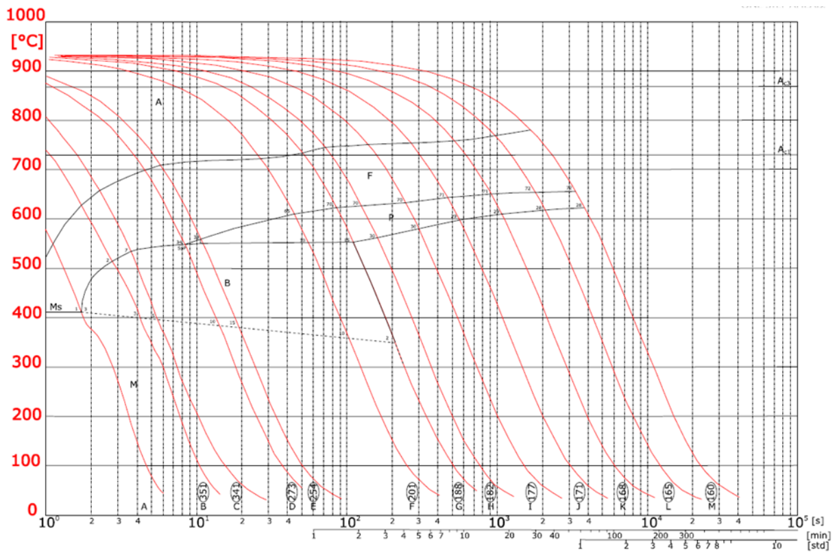
Figure 3-10: CCT Diagram: Dilatometer laboratory measurement of Steel Grade B: 40 \mu\text{m} austenite grain size (austenitized at 930 °C)
