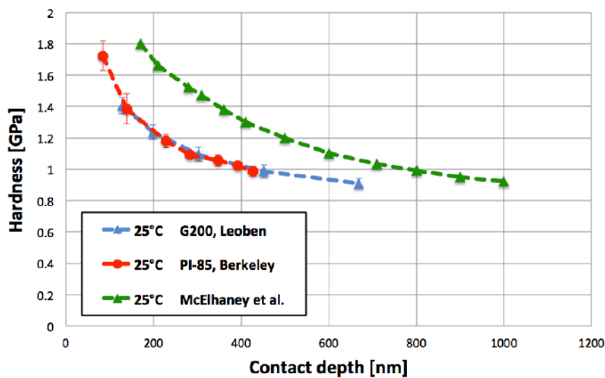
Fig. 4.7: Comparison of room temperature hardness values of sx Cu: PI-85, Berkeley, G200, Leoben and McElhaneý's investigations [33].
