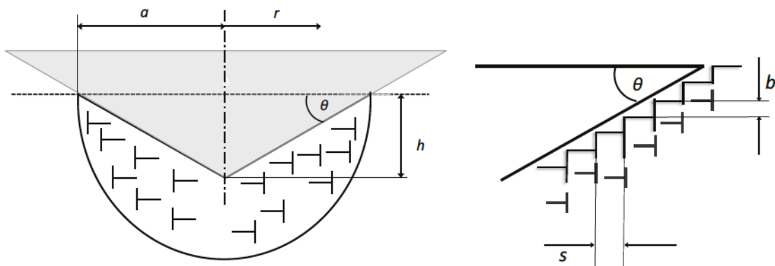
Fig. 2.7: Geometrically necessary dislocations created by a rigid conical indentation. The dislocation structure is idealized as circular dislocation loops.
