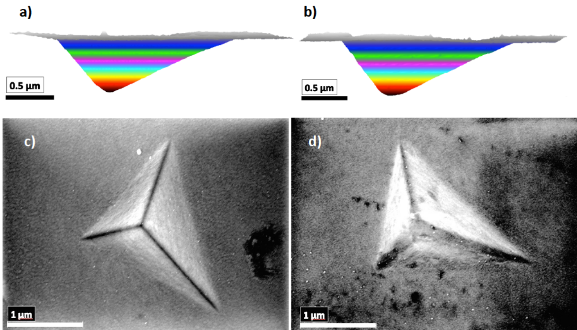
Fig. 4.26: AFM image of indent on sx W with 10 mN, showing the altered tip with tip radii of a) 125 nm and b) 530 nm. c) and d) correlating SEM images
