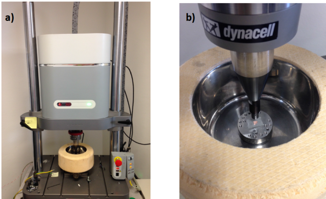
Fig. 3.2: a) Universal testing device "INSTRON E3000", b) sx Cu sample on cool-able stage
