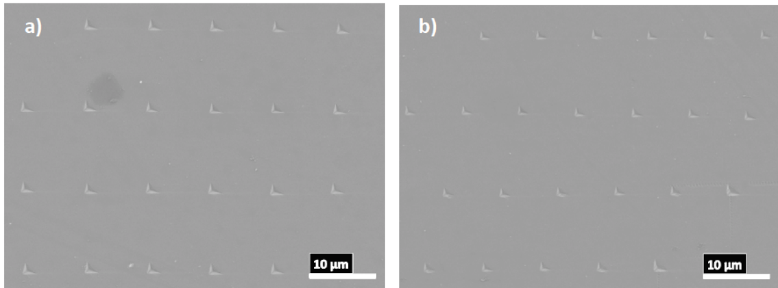
Fig. 4.21: Array of indents performed for the pop-in investigations on sx W at a) RT and b) -150^\circ\text{C}
