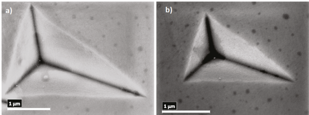
Fig. 4.10: SEM images of 10 mN indents on sx Cr at a) RT and b) -150^\circ
