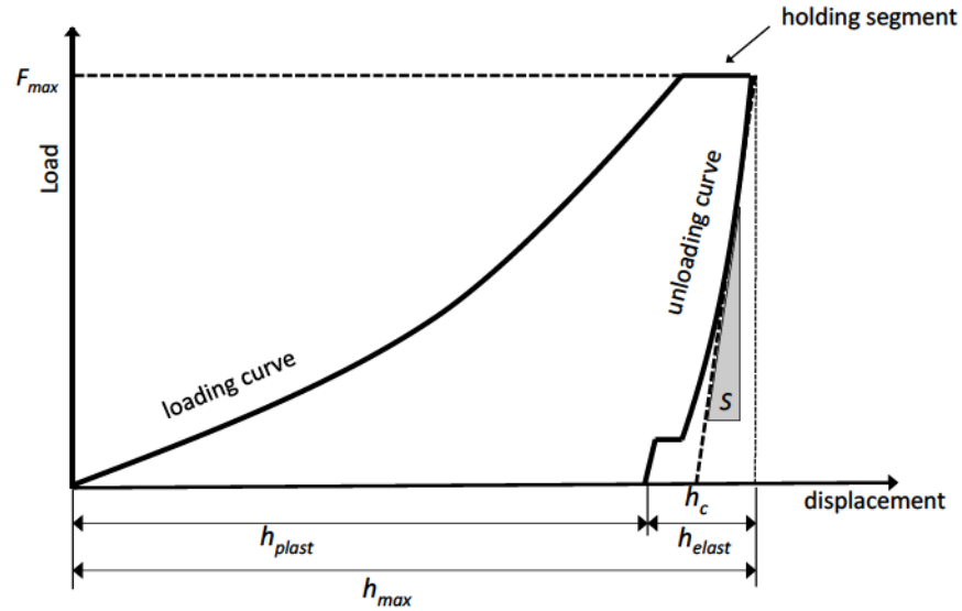
Fig. 2.3: Load displacement curve of nanoindentation testing
