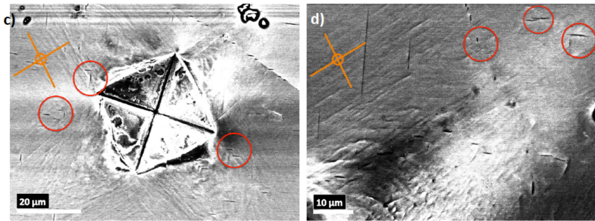
Fig. 4.5: SEM image of 5 N Vickers indents on sx Cr at a) RT and b) -196°C, both showing [1 1 0] slip planes. Perpendicular micro-cracks around the imprint at c) -196°C and d) RT
