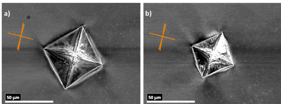
Fig. 4.6: SEM images of sx W with 5 N Vickers indents at a) RT and b) -196°
