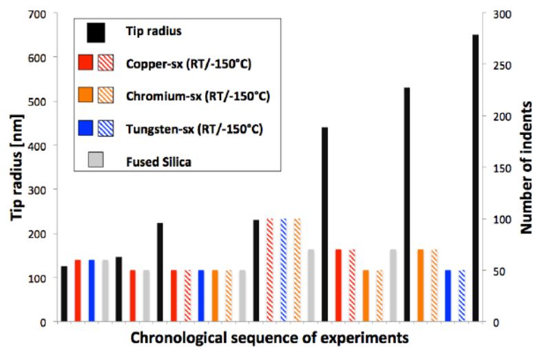
Fig. 4.25: Tip alteration over the scope of experiments
