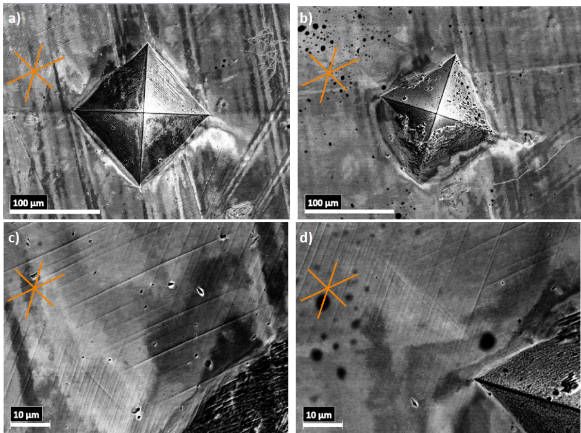
Fig. 4.4: SEM images of 5 N Vickers indents on sx Cu at a) RT and b) -196^\circ\text{C} . c) and d) show the correlating slip planes, both obtaining [1 1 1] direction.
