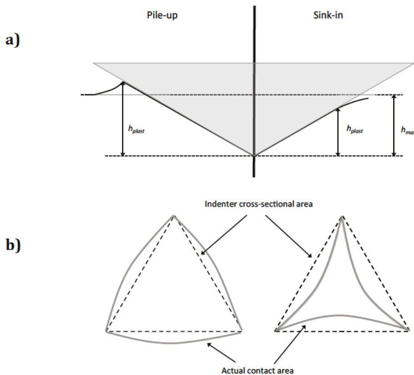
Fig. 2.5: Projections of pile-ups and sink-ins. a) cross-sectional projection. b) plan view projection.
