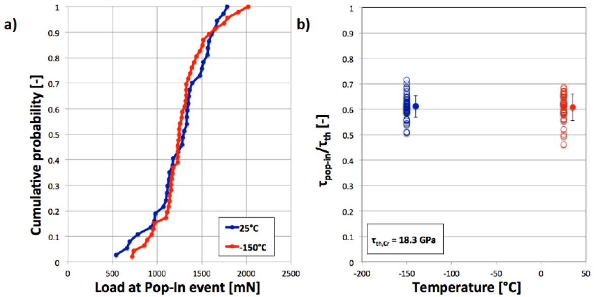
Fig. 4.23: a) Comparison of cumulative probability of pop-ins appearing versus corresponding pop-in load at different temperatures of sx Cr. b) Theoretical strength versus temperature.
