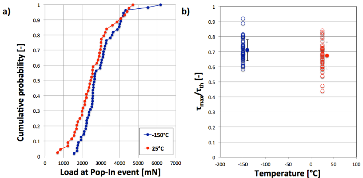
Fig. 4.24: a) Comparison of cumulative probability of pop-ins appearing versus corresponding pop-in load at different temperatures of sx W. b) Theoretical strength versus temperature.
