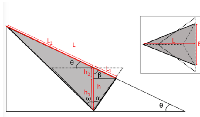
Fig. 5.3: Scheme of a print obtained by nanoindentation on a tilted surface according to Laurent-Brocq. Cross view and top-view (right corner) [81]
