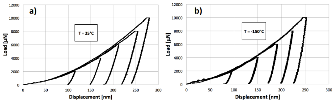
Fig. 4.13: Material response of sx W at a) room temperature and b) -150^\circ\text{C} at different load levels
