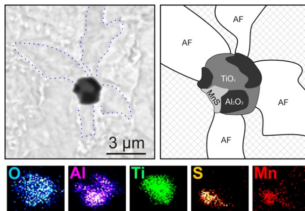
Figure 12: Non-metallic inclusion that acts as nucleus for acicular ferrite in steel A.
