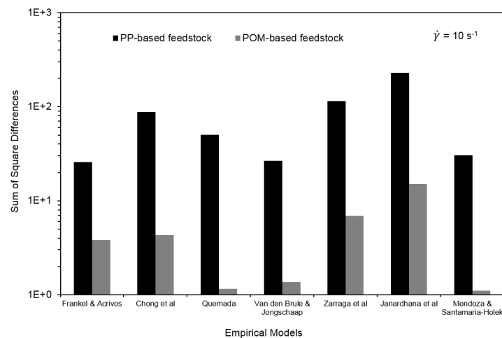
Figure 8. Square difference for models of viscosity as a function of powder loading for PP-based feedstock viscosity at 170 \text{ }^{\circ}\text{C} and POM-based feedstock viscosity at 180 \text{ }^{\circ}\text{C} . Only models with maximum one fitting parameters are shown here.
